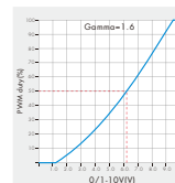
0/1-10V dimming
